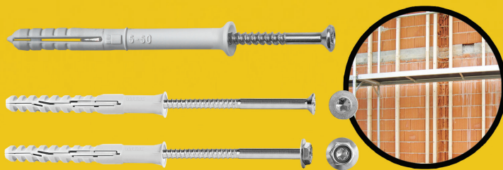
FRAME PLUGS 8mm & 10mm length 60mm - 240mm
