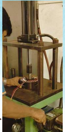
SHAFT FIXING (HYDRAULIC)
